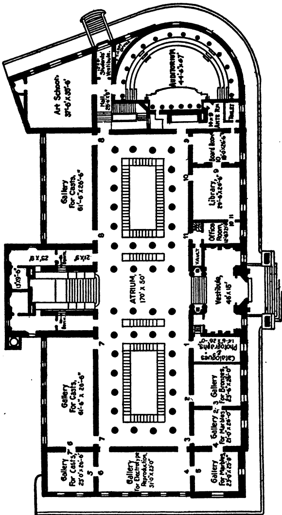
PLAN OF FIRST STORY
